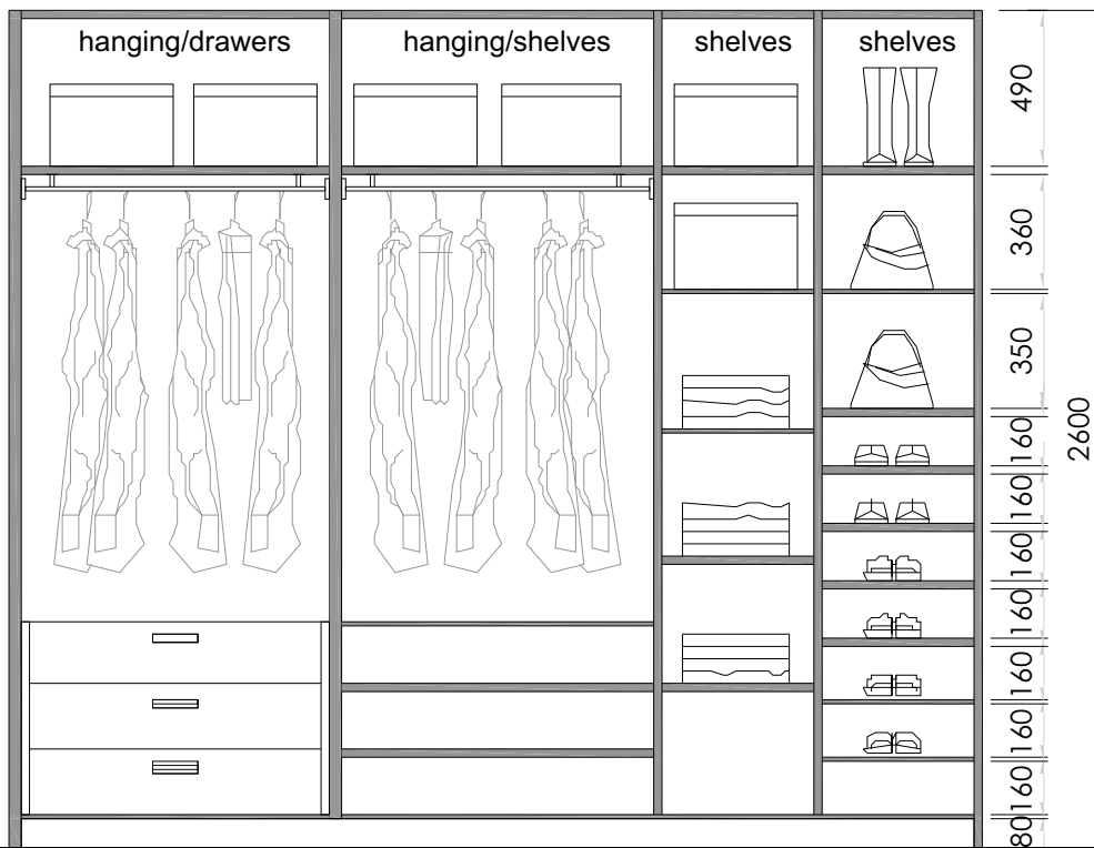
INTERIOR ELEVATION
